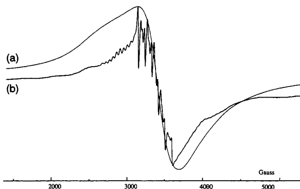
Figure 6. X-band DMF/toluene glass EPR spectra of (Mn 2 HL 3 (CH 3 -CO 2 ) 2 (CH 3 OH)) 2 (3) at 90 K before (a) and after (b) reaction with O 2 (O 2 :3 ratio ~ 1:2; microwave power 20 mW; microwave frequency 9.4225 GHz (a), 9.4264 GHz (b); 10-G modulation amplitude).
